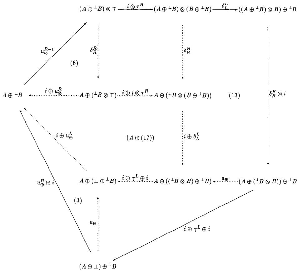
Fig. 2. Triangle identity.
